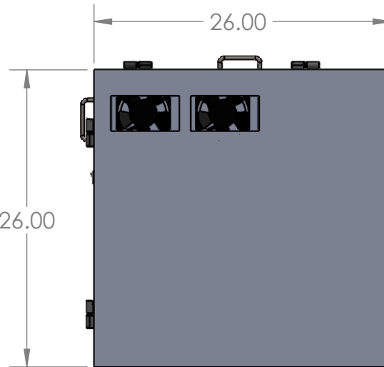
RIGHT VIEW
