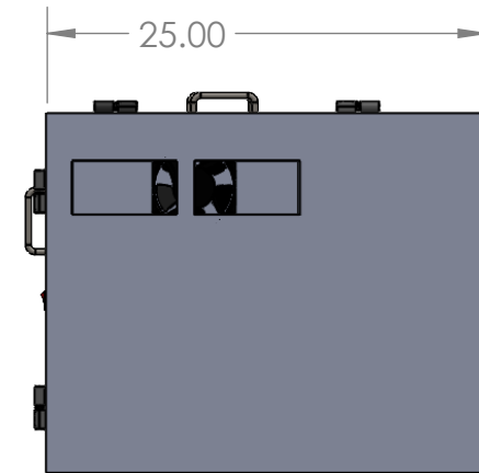
RIGHT VIEW
