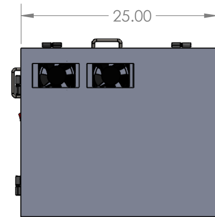
RIGHT VIEW
