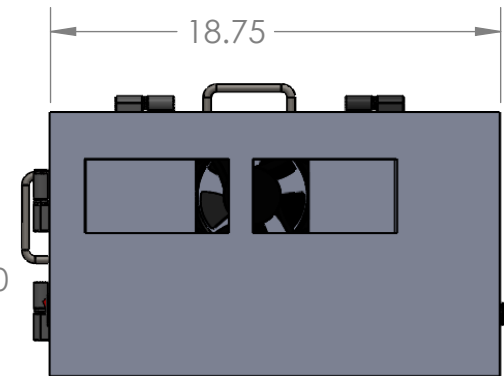
RIGHT VIEW
