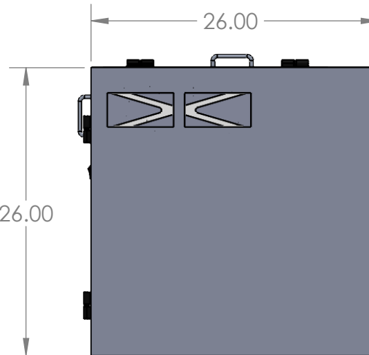
RIGHT VIEW
