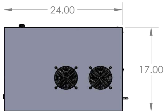
LEFT VIEW
