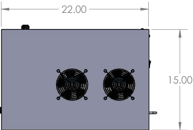
LEFT VIEW
