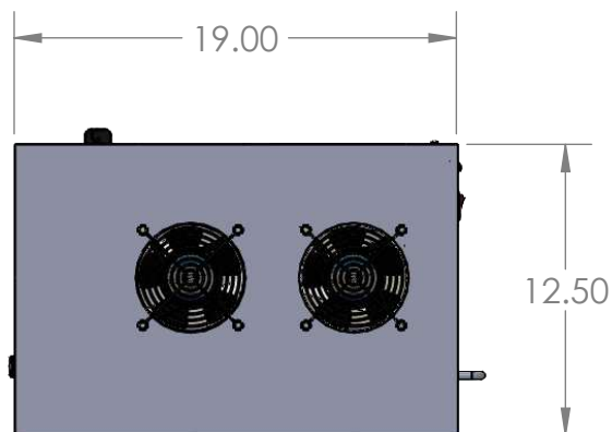
LEFT VIEW
